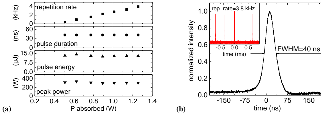
Fig. 2. Repetition rate, pulse duration, output energy and peak power of the PQS Tm,Ho:YLF laser vs. absorbed pump power for T_{OC}=1.5\% (a) and Q-switched pulse shape and pulse train (inset) (b).
