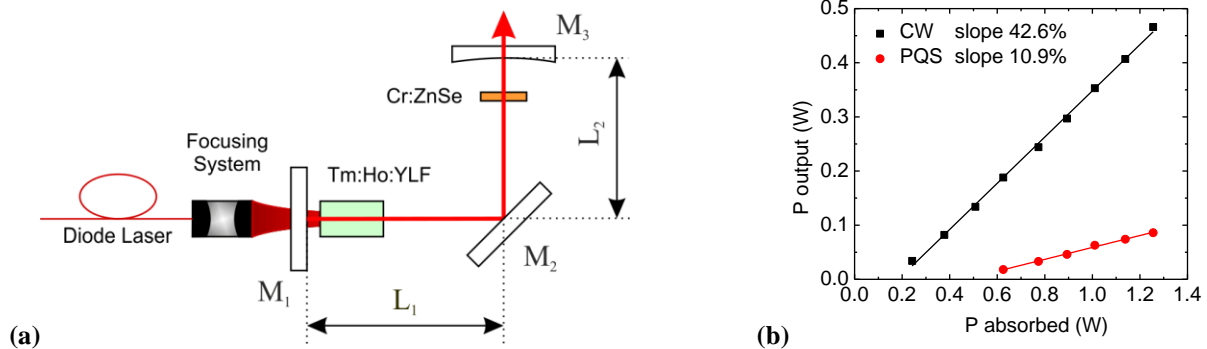
Fig. 1. (a) Setup of the PQS Tm,Ho:YLF laser. M 1 : dichroic pump mirror, M 2 : HR-laser, HT-pump mirror, M 3 : output coupler. (b) Output power vs. absorbed pump power for 5.8% OC in CW and PQS regimes.
