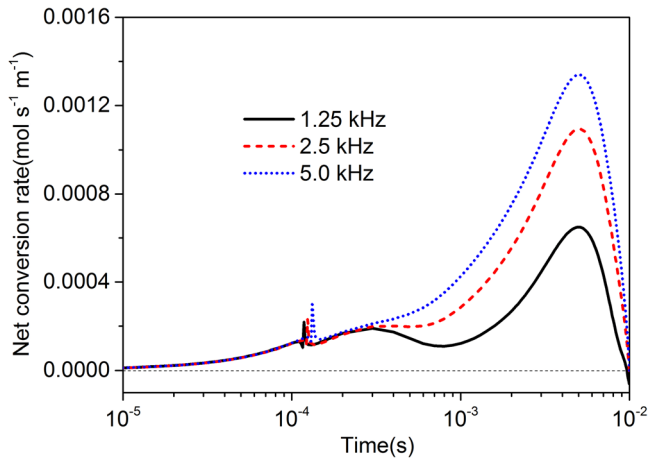
Figure 12. Time evolution of the spatially integrated net conversion rate of \text{CO}_2 for different frequencies of convective cooling, at the same condition as in figure 10.
