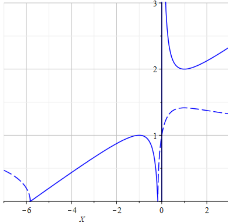
Fig. 1. Plot of R/r_s (solid) and M_0/M (dash) as a function of the factor X
